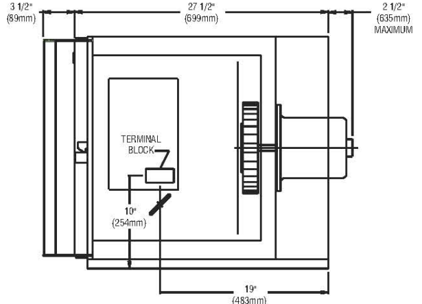
Side View – Single Unit
