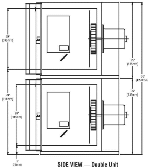
SIDE VIEW — Double Unit
