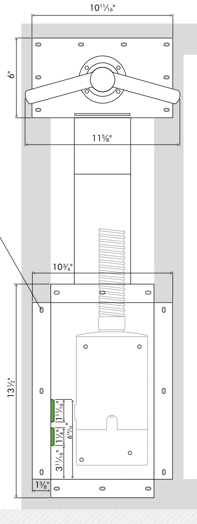
REAR ELEVATION
